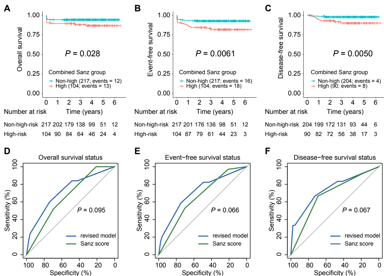
Figure S15. Kaplan–Meier plots of Combined Sanz groups and ROC plots between the Sanz score and the revised risk score. Kaplan–Meier estimates of OS (A), EFS (B), and DFS (C) when combining the Sanz low- and intermediate-risk into a single category. Comparison of the OS (D), EFS (E), and DFS (F) ROC curves between the Sanz score and the revised model score. P -value is calculated using the log-rank test. OS, overall survival; EFS, event-free survival; DFS, disease-free survival; ROC, receiver operating characteristic.
