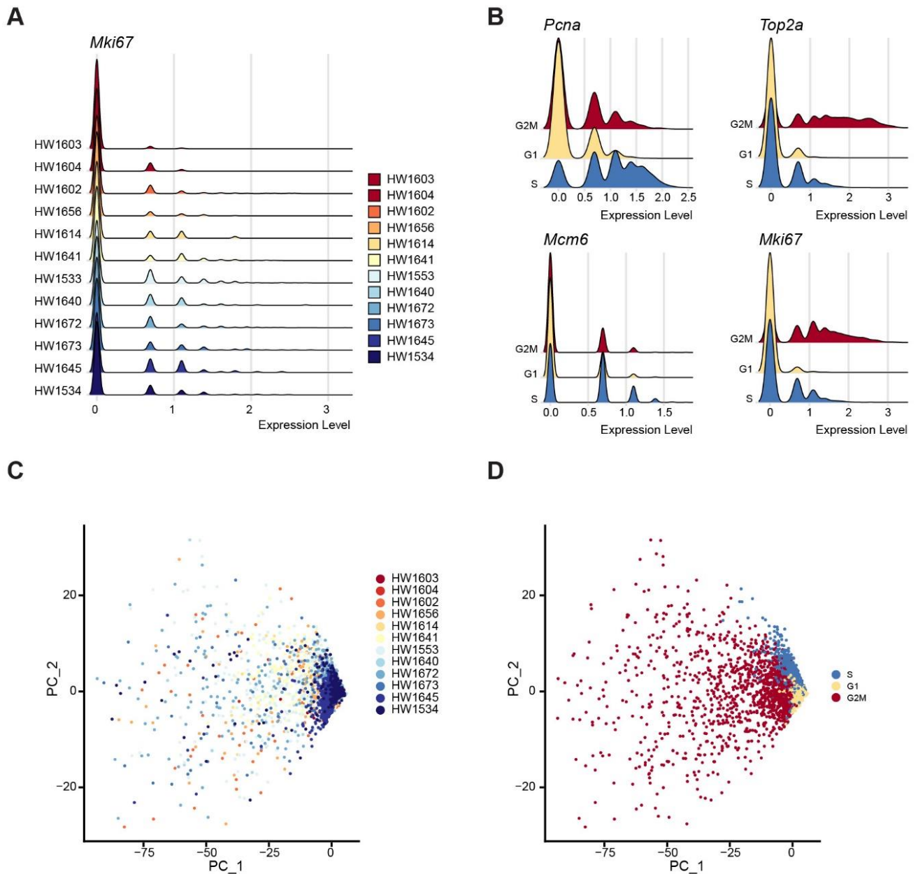
Supplementary Figure S5 | Cell cycle stage assignment of the SCLC cells from the autochthonous model. A , Mki67 expression of the SCLC cells. B , Reliability of the cell cycle stage assignment by the markers ( Pcna , Top2a , Mcm6 , Mki67 ). Principal component plot of the autochthonous SCLC cells labeled by (C), and by cell cycle stage assignment (D).
