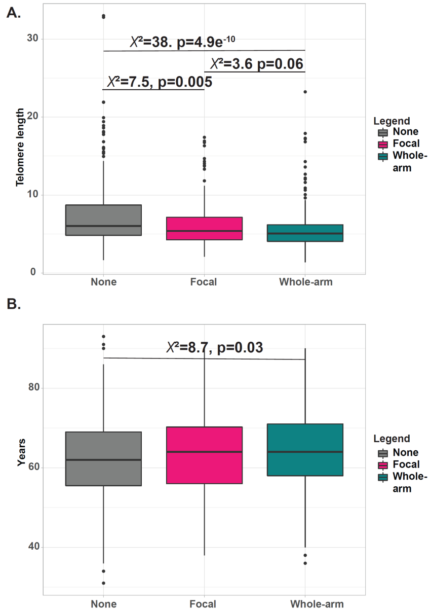
Supplemental Figure 10. Correlation between age, telomere length and 1q gain subtype. A. Correlation between telomere length and chromosome 1 rearrangement subtype B. Correlation between age and chromosome 1 rearrangement subtype
