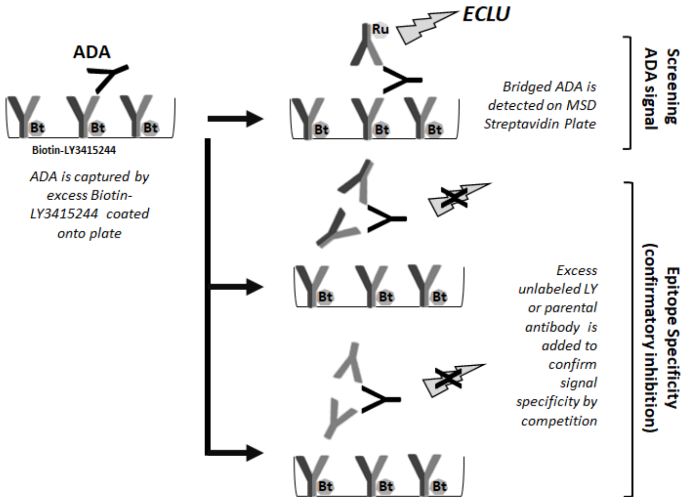
Supplemental Figure 1. Generation of the screening ADA signal and confirmatory inhibition by the affinity-capture elution-bridge assay format
