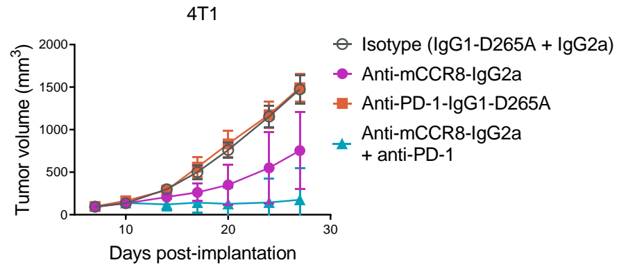
Supplemental Figure 7: Mean growth curves of subcutaneous 4T1 (n= 10 per group) tumors treated with isotype control antibodies, anti-mCCR8-IgG2a, anti-PD-1, or the combination of anti-mCCR8-IgG2a and anti-PD-1 antibodies at 0.2 mg/mouse/treatment at day 7, 10 and 14 after tumor implantation.
